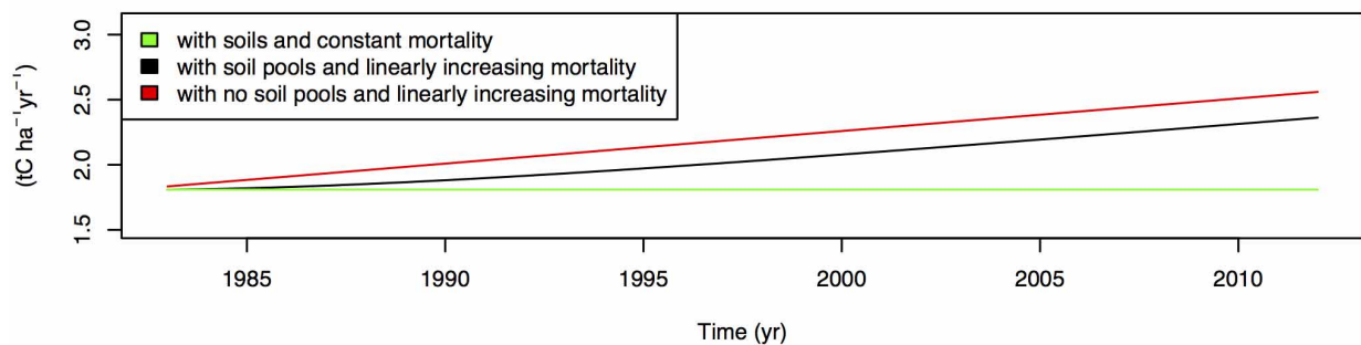
Extended Data Figure 10 | Modelled estimates of the effects of linearly increasing mortality on necromass stocks and soil organic-matter stocks. a , Necromass stocks. b , Soil organic matter stocks. c , The estimated fluxes of carbon from the forest to the atmosphere in three scenarios: (1) assuming constant mortality rate and a lag in decomposition of dead-tree biomass
